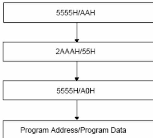
Figure 6-3.Embedded Programming Algorithm State Diagram
