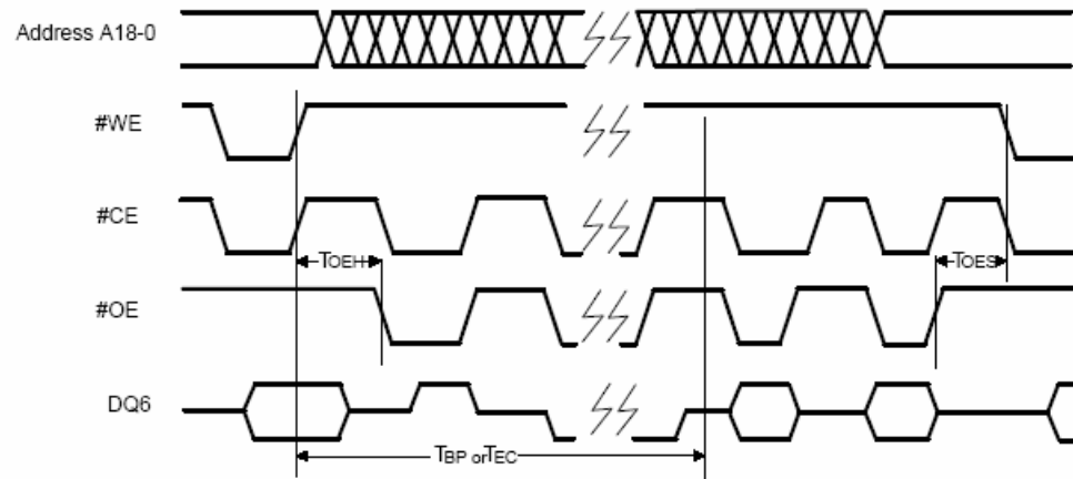
Figure 6-12.Toggle Bit Timing Diagram
