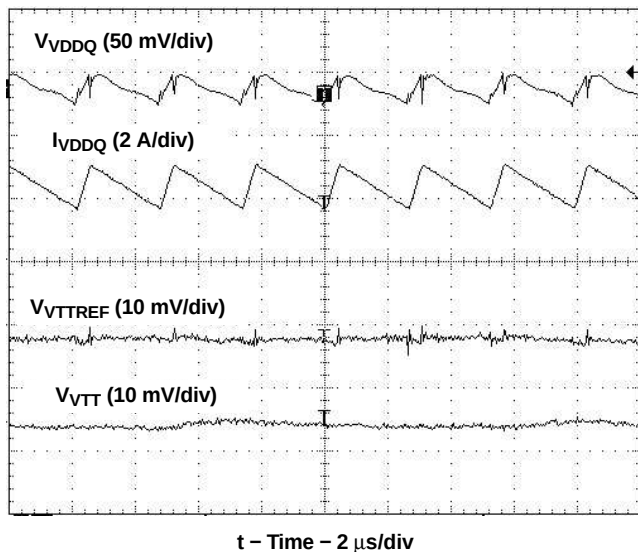
Figure 24. Ripple Waveforms - Heavy Load Condition
