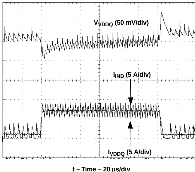
Figure 25. VDDQ Load Transient Response
