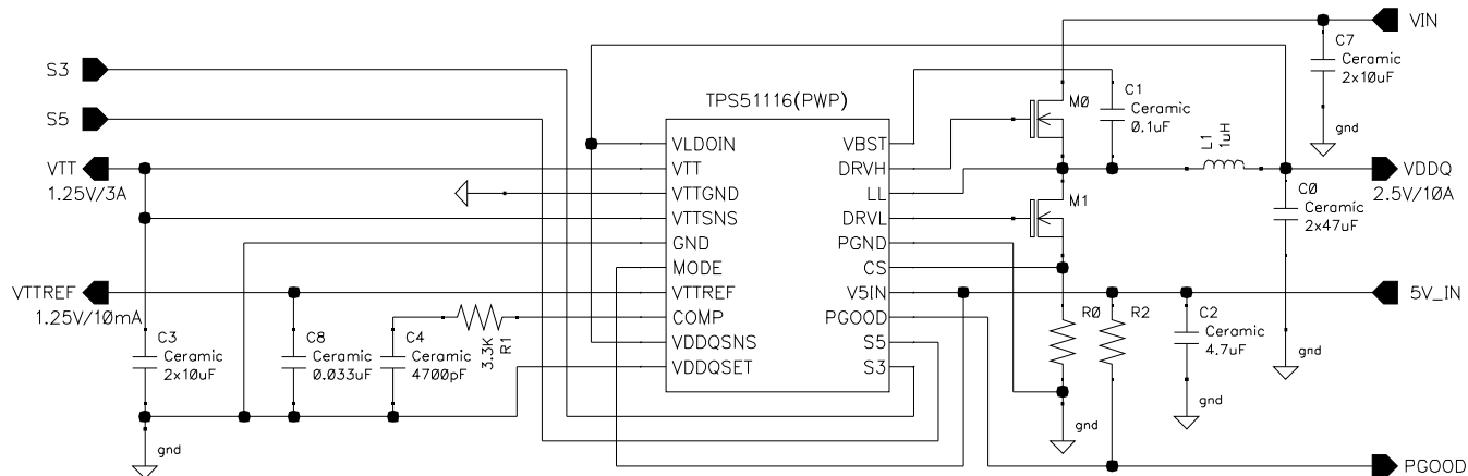
Figure 5. Current Mode
