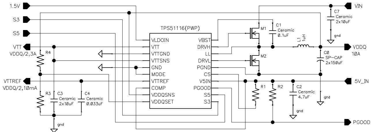
Figure 4. D-CAP™ Mode
