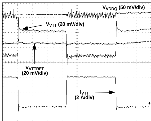
Figure 26. VTT Load Transient Response
