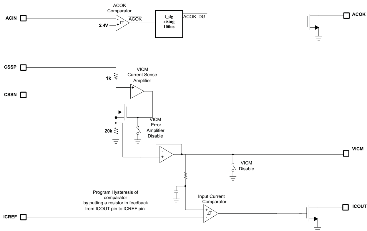
Figure 31. ACOK, ICREF, and ICOUT Logic
